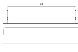
Suspended luminaires
